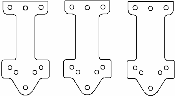
H, J, K - M12, M15, M18-150WB G10 Rear Tuning Pods
